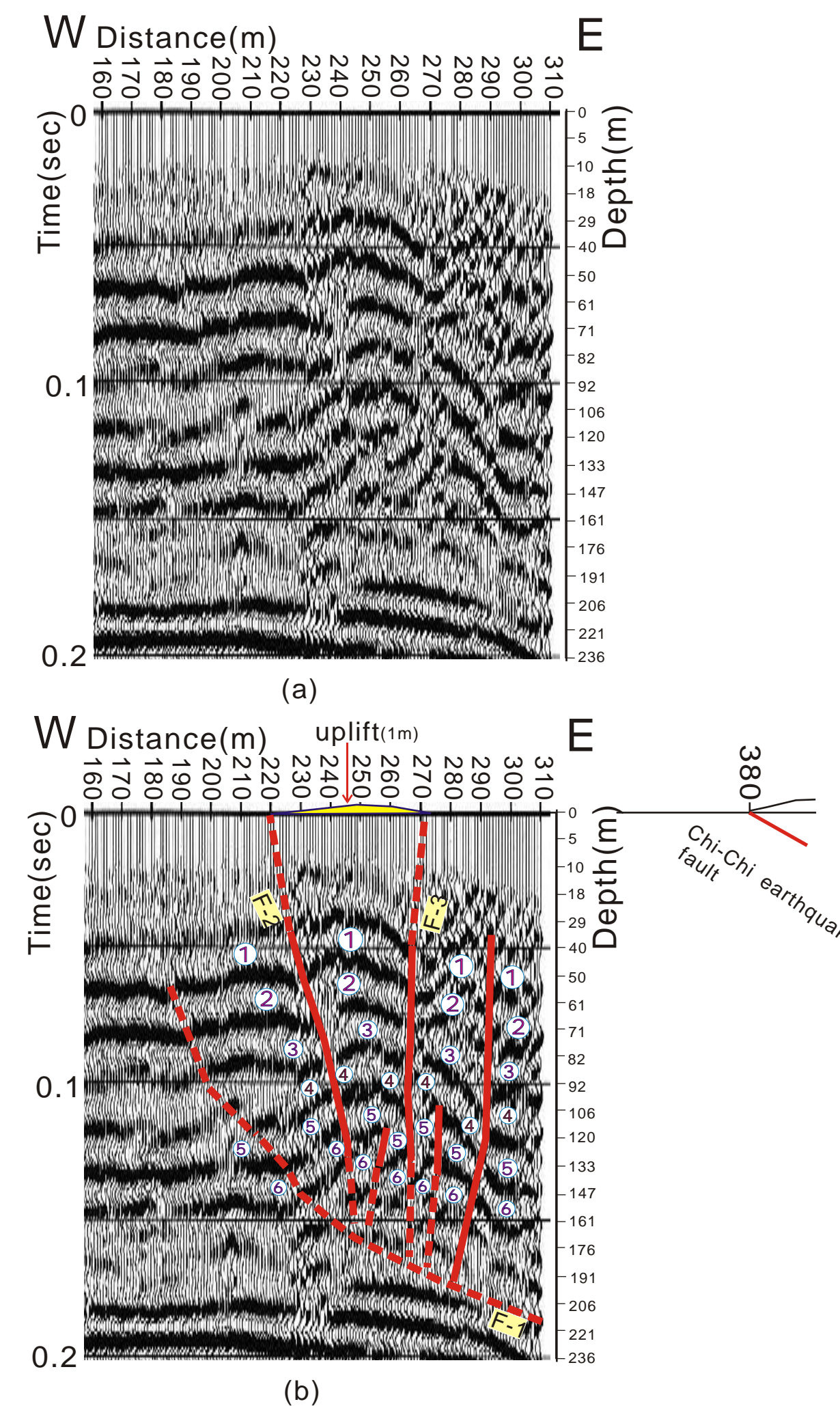
The high-resolution seismic section of downthrown block at Chelungpu fault zone in Wufeng area.
