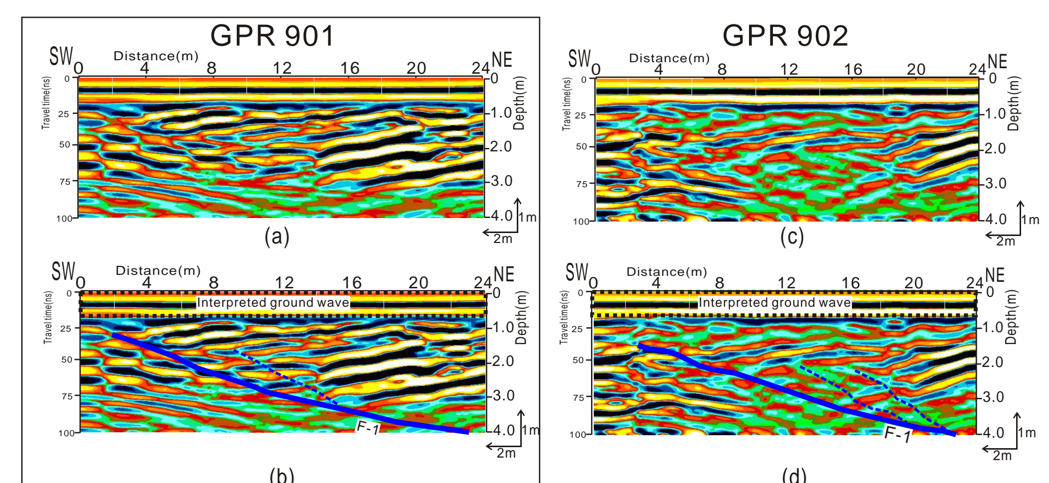
GPR profiles of Chelungpu fault in Wufeng area.
