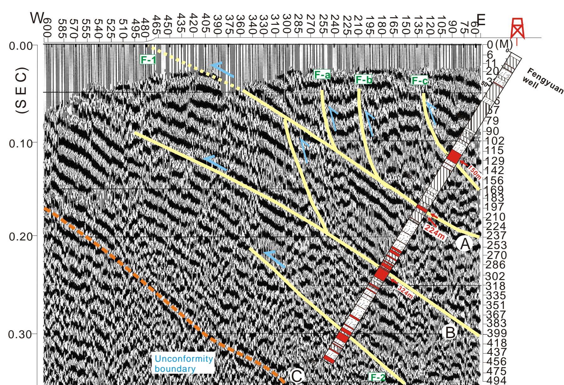
The correlation of high resolution seismic section and drilling well at Chelungpu fault. The correlation indicates the prediction of seismic data was correct.
