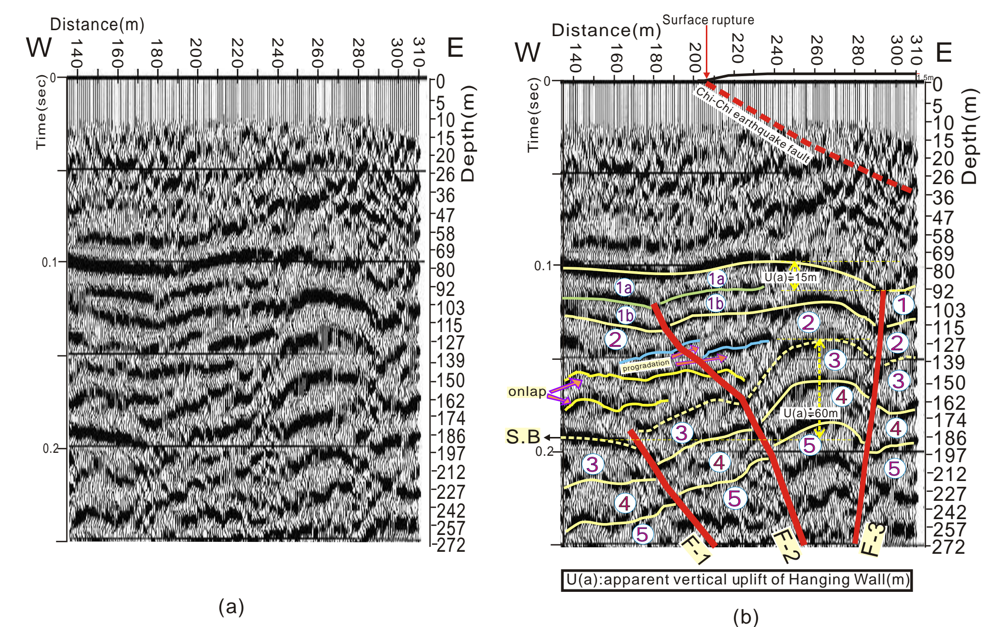
The high-resolution seismic section of Chelungpu fault zone in Wufeng area at grape yard
