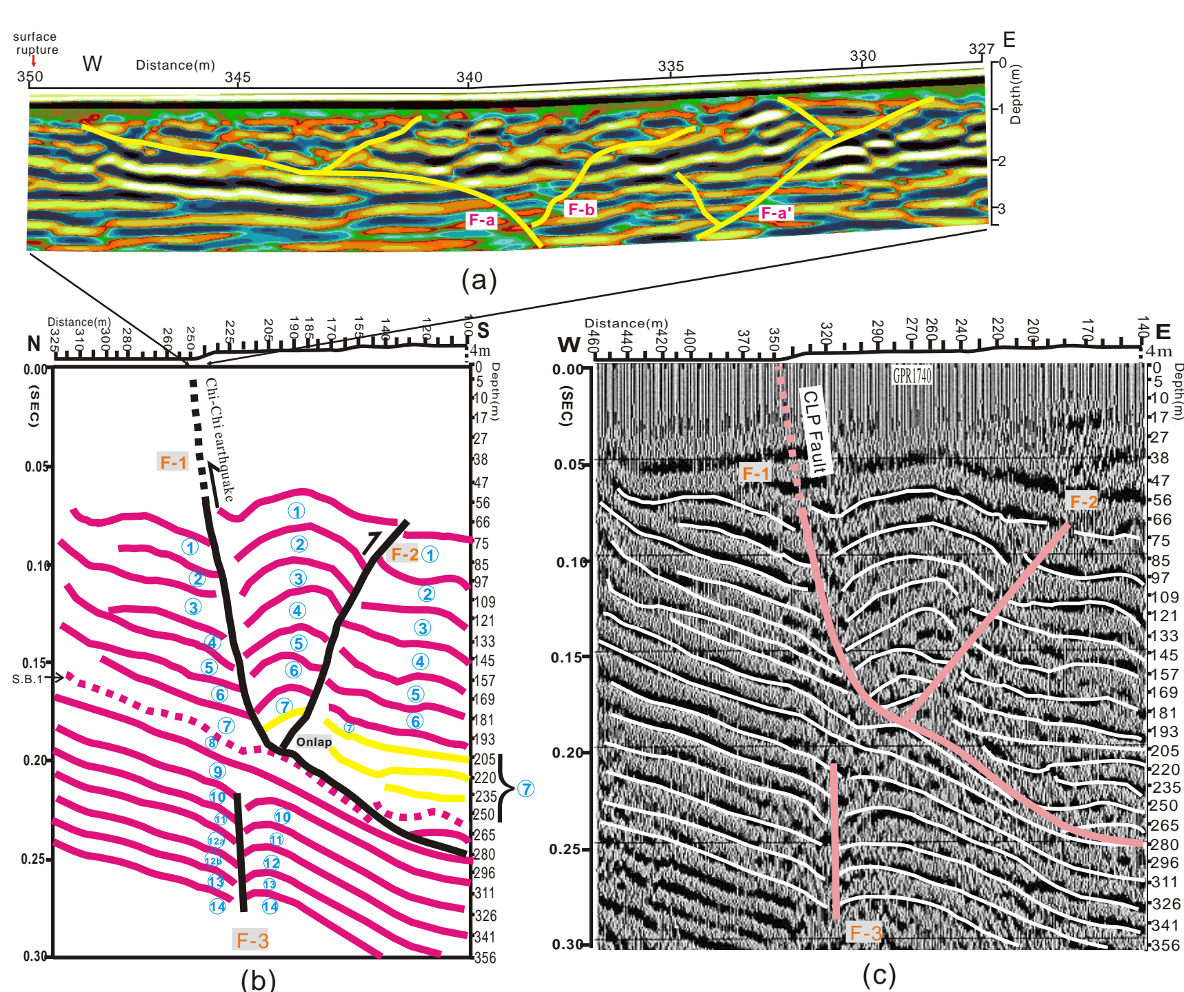
The GPR profile and seismic section of Chelungpu fault in Shihkang area.
