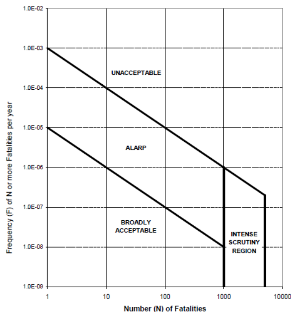
Figure 2. F-N Curve for Evaluating Societal Risk.
