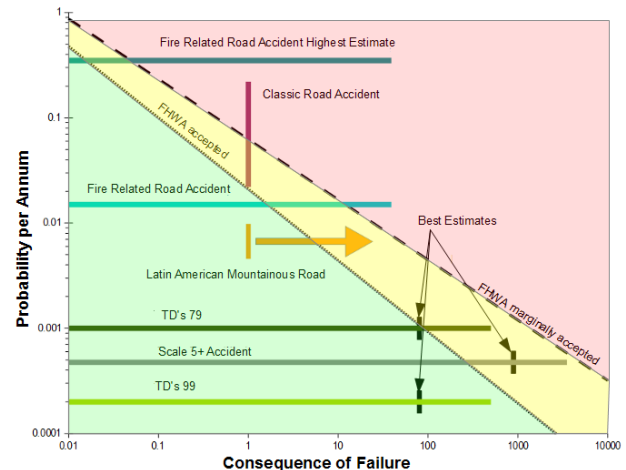
Figure 3. Various accidents (consequences are casualties only) compared to FHWA/Whitman societal tolerability curves. The black vertical traits represent the position of the consequences best estimates (Oboni, Oboni, 2013).
