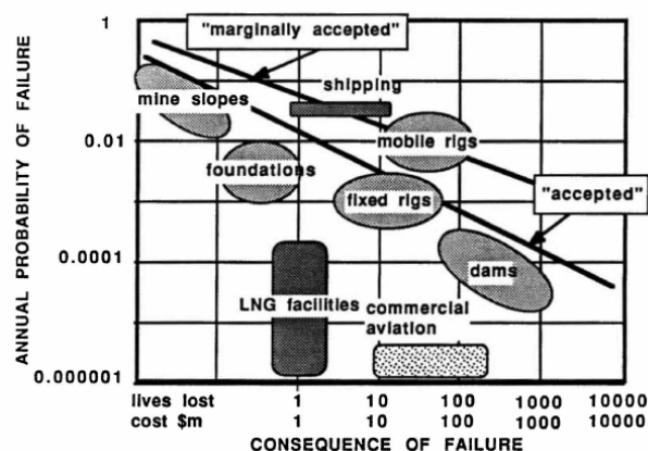
Figure 1. Empirical rates of failure for civil facilities.
