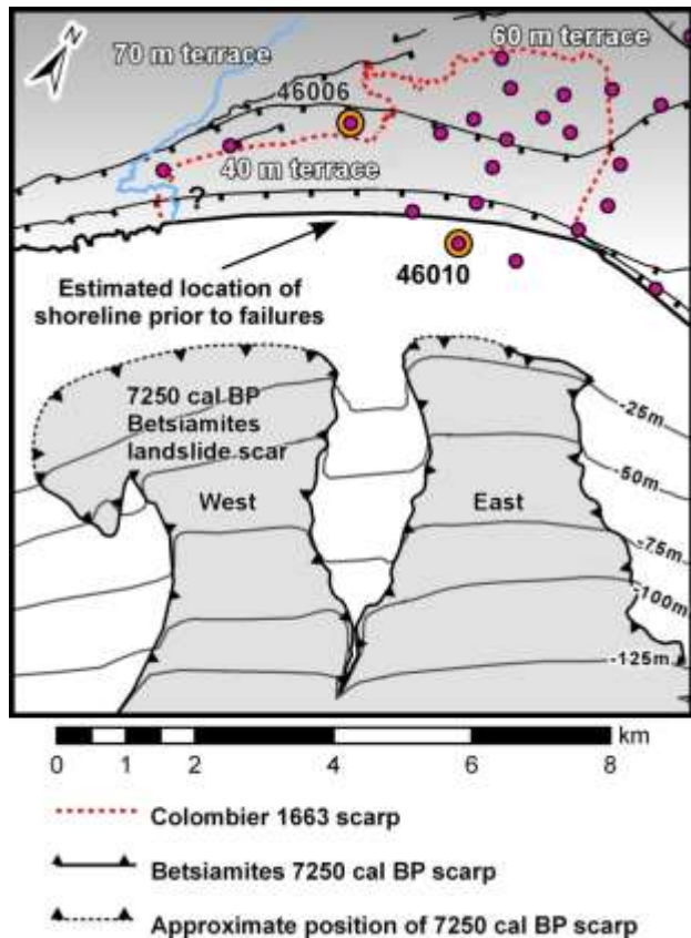
Figure 6. Interpreted topography prior to the 1663 Colombier slide event (see Figs. 2 and 3 for symbols definition).
