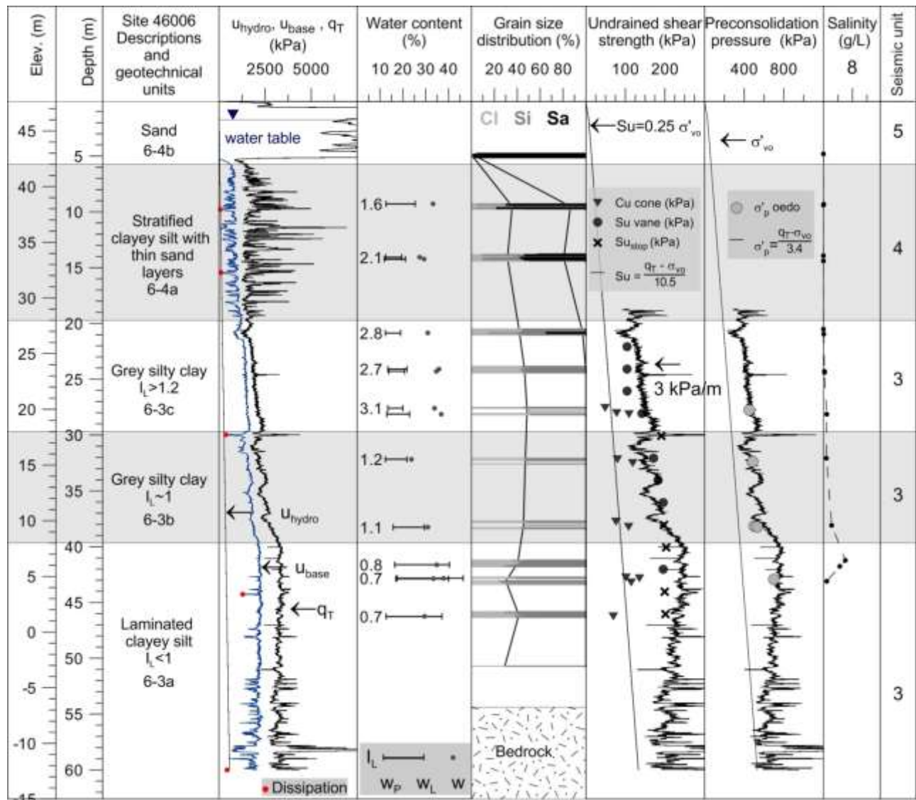
Figure 8. Geotechnical properties of borehole 46006.
