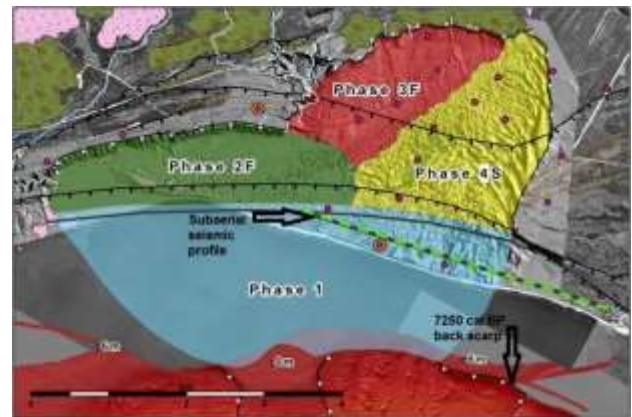
Figure 7. Landslide extent and failure phases of 1663 Colombier slide event. The Colombier slide event involved four successive failure phases: one submarine and three subaerial (see Figs. 2 and 3 for symbols definition).
