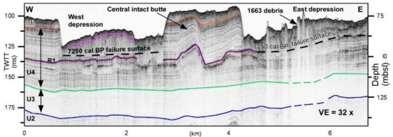
Figure 4. Seismic profile across the butte showing the various stratigraphic units and the accumulation of debris in both depressions and on the butte (see Fig. 2 for the location of the seismic line). Units U2 to U4 are also described on the geotechnical profiles in Figs. 5 and 8.
