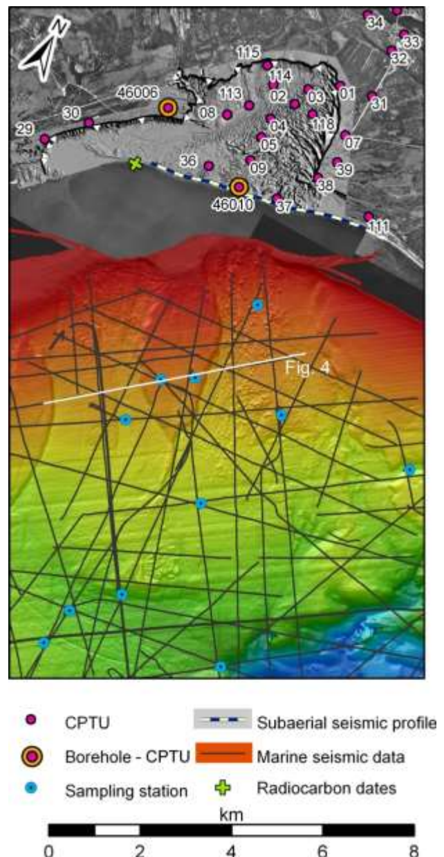
Figure 2. Investigation carried out in the subaerial and submarine area of the Betsiamites-Colombier slides. Numbers refer to CPTUs and 46006 and 46010 to boreholes.
