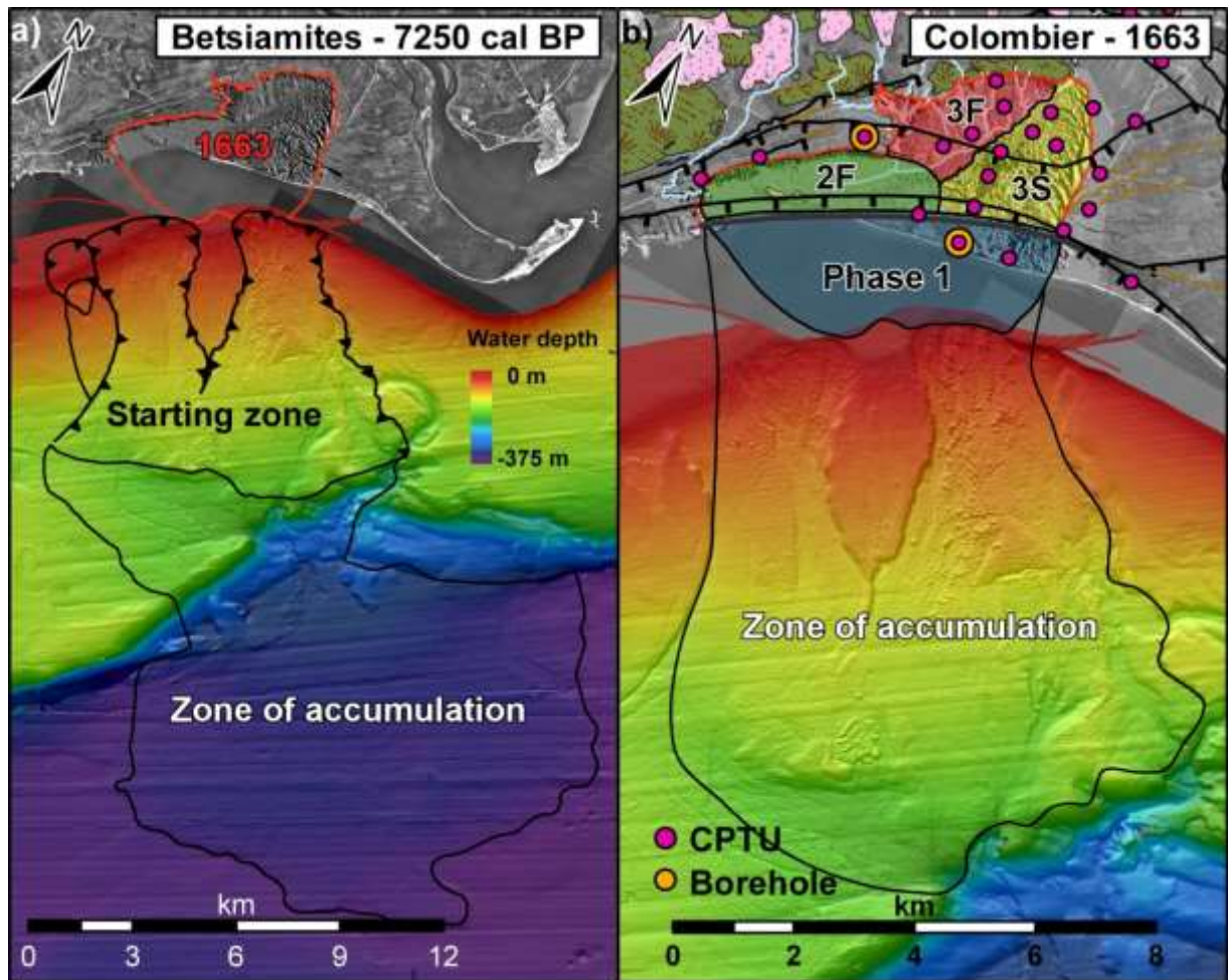
Figure 3. Boundaries of the Betsiamites-Colombier slides (see Figure 2 for symbols definition).
