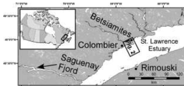
Figure 1. Map of the study area
