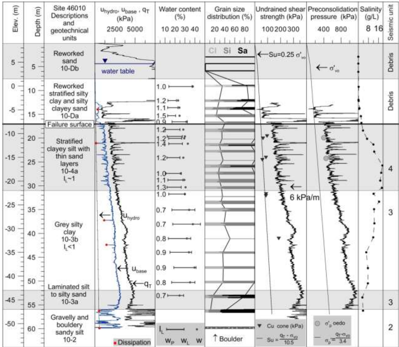
Figure 5. Geotechnical properties of borehole 46010.
