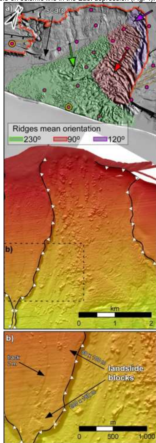
Figure 9. Morphology of the debris within the landslide scars. a) Arrows indicate the direction of the movements of the subaerial ridges. b) Subaerial blocks dispersed underwater. On the central butte, the blocks produced an erosion glide track about 1-2 m deep. (see Fig. 2 for symbols definition).
